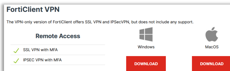
Abbildung 1: FortiClient Download
